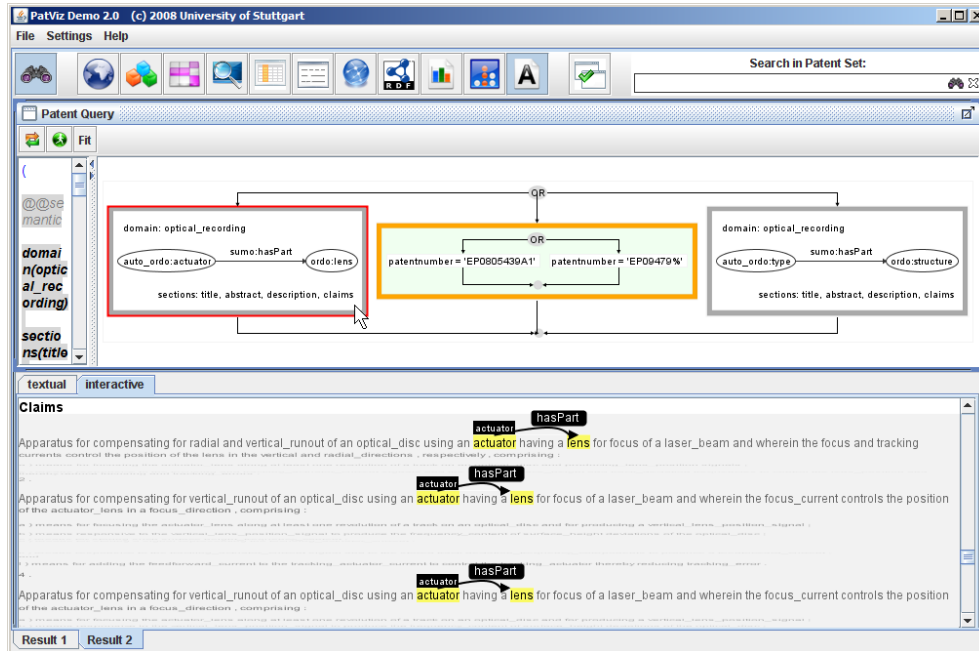
Figure 2: Highlighting of Semantic Search Results and Metadata Structure
