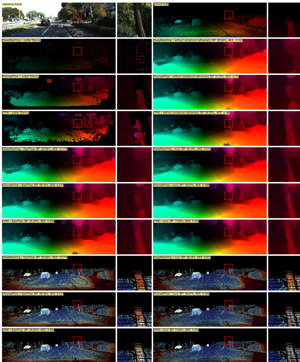
Figure 5.6: Results for the sequence #31 of the KITTI 2015 benchmark [119]. First row: Reference frame and ground truth. Second to fourth row: Outlier-filtered matches and inpainted matches (DeepMatching, DiscreteFlow, CPM). Fifth to seventh row: Flow field visualization of the EpicFlow refinement and proposed refinement (DeepMatching, DiscreteFlow, CPM). Eighth to tenth row: Error visualization of the EpicFlow refinement and our refinement (DeepMatching, DiscreteFlow, CPM).
