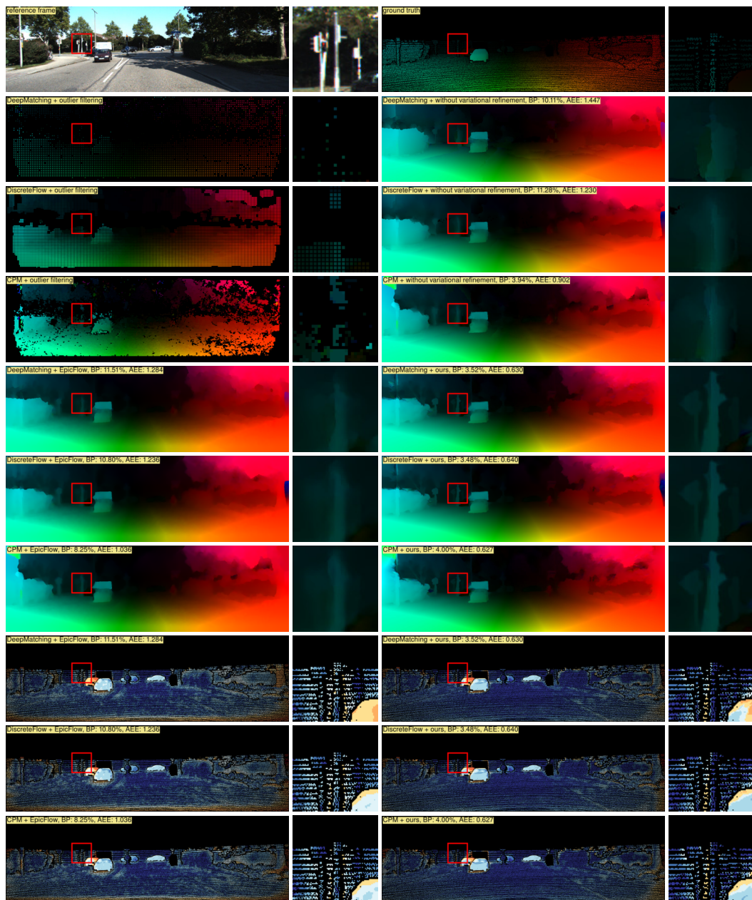
Figure 5.5: Results for the sequence #07 of the KITTI 2015 benchmark [119]. First row: Reference frame and ground truth. Second to fourth row: Outlier-filtered matches and inpainted matches (DeepMatching, DiscreteFlow, CPM). Fifth to seventh row: Flow field visualization of the EpicFlow refinement and proposed refinement (DeepMatching, DiscreteFlow, CPM). Eighth to tenth row: Error visualization of the EpicFlow refinement and our refinement (DeepMatching, DiscreteFlow, CPM).
