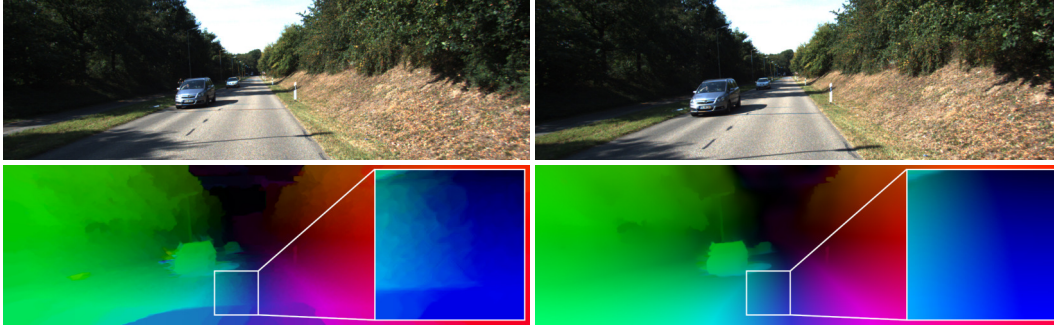
Figure 1.2: Different regularization order for motion estimation. Top to bottom, from left to right: (a-b) Input images [119]. (c) Motion field computed using a first-order regularizer. (d) Motion field computed using a second-order regularizer.
