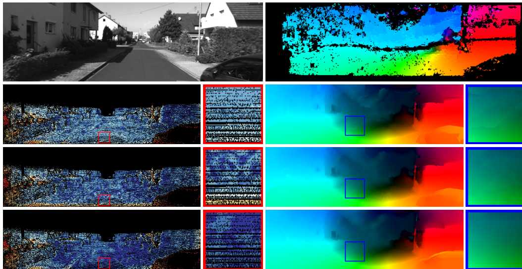
Figure 5.2: Training sequence #28 of KITTI 2012 [65]. First row : Reference image, CPM matches. From left to right : Error and motion field visualization. Second row : Inpainted CPM matches (BP: 7.86%). Third row : EpicFlow refinement (BP: 10.80%). Fourth row : Proposed refinement (BP: 7.03%).
