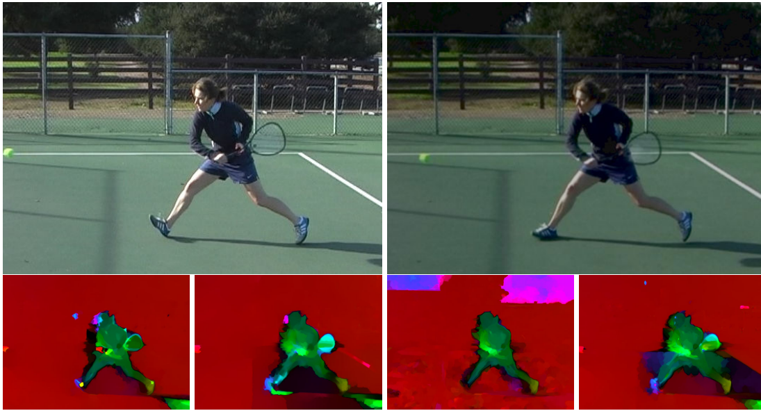
Figure 6.5: Results for Tennis sequence with artificial illumination changes. From Left To Right: (a) Gradient constancy assumption (GCA). (b) Geometric Blur constancy assumption (GBCA). (c) Complete Rank Transform (CRT). (d) BCA and GCA after illumination compensation.
