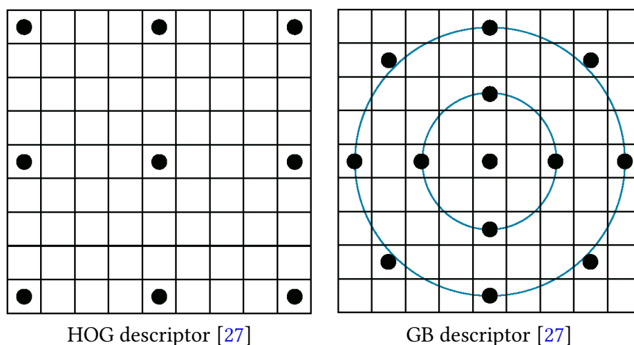
Figure 2.3: The blocks that are used in the HOG and the GB descriptor.
