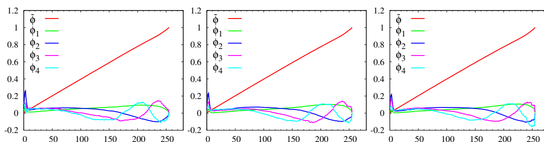
Figure 5.3: Impact of iterating the estimation of the KITTI 2012 basis functions. From left to right: (a) Initial basis. (b) After one iteration. (c) After four iterations.
