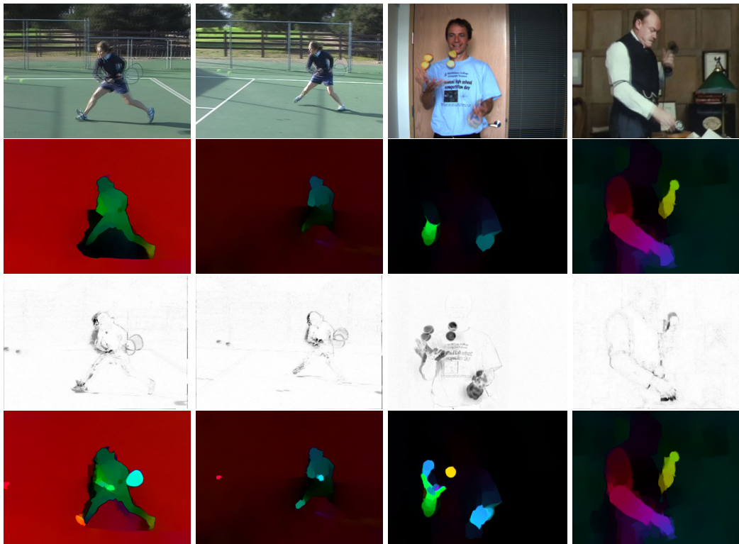
Figure 3.6: Condensed overview of the flow estimation for different large displacement sequences. From Left to Right: Tennis sequence (Frames 496 and 577), Beanbags sequence (Frame 10), Miss Marple sequence (Frame 52). From Top to Bottom: (a) Overlaid input images. (b) Initial flow field without feature matches. (c) Local energy of the data term (registration error). (d) Final result of our method.
