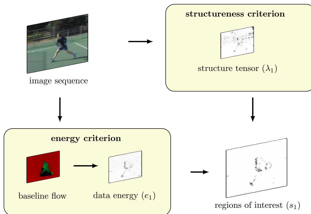
Figure 3.3: Illustration of the selection criteria. Thresholding the smaller eigenvalue \lambda_1 of the structure tensor of the first frame indicates sufficient structuredness for a feature descriptor while thresholding the data energy e_1(\mathbf{x}) of the baseline indicates the need for additional guidance by feature matches. The combination of both gives us the regions of interest for feature matching. Here, dark colors indicate high values.
