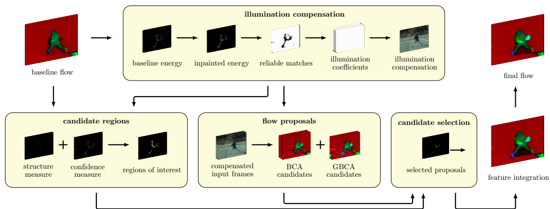
Figure 6.6: Schematic overview of the completely decoupled method ( ICALD ) at hand of the Tennis sequence [27].
