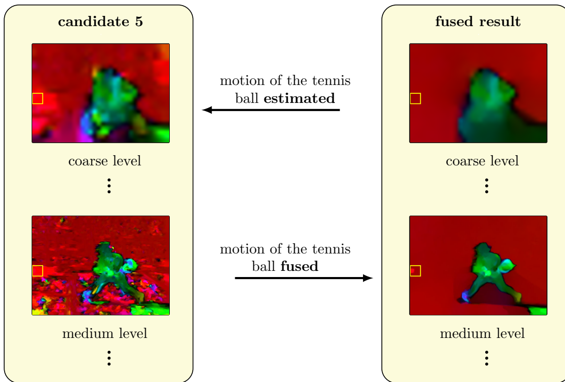
Figure 4.6: Estimation and fusion of the large displacement of the tennis ball from the Tennis sequence (Frame 496) [27]. While the corresponding candidate motion is estimated at a coarse level, the fusion into the final result is done at a medium level.
