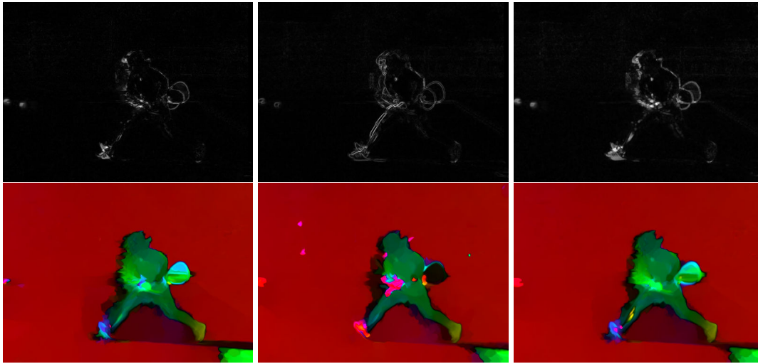
Figure 4.10: Effect of different data constancy assumptions on the final result. From left to right: Brightness constancy assumption (BCA), Gradient constancy assumption (GCA) and both combined. From top to bottom: Data costs of the baseline flow (brighter grey values indicate larger energies), final result.
