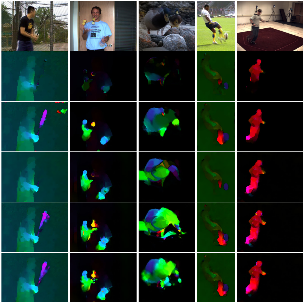
Figure 4.7: Comparison of LDOF and our method with the corresponding baseline results. Left to right: Baseball sequence [160], Beanbags sequence [9], Bird sequence, Football sequence [160], Human Eva sequence [123]. Top to down: Overlaid frames, LDOF baseline, LDOF, our baseline, our result, our result (LDOF regularizer).
