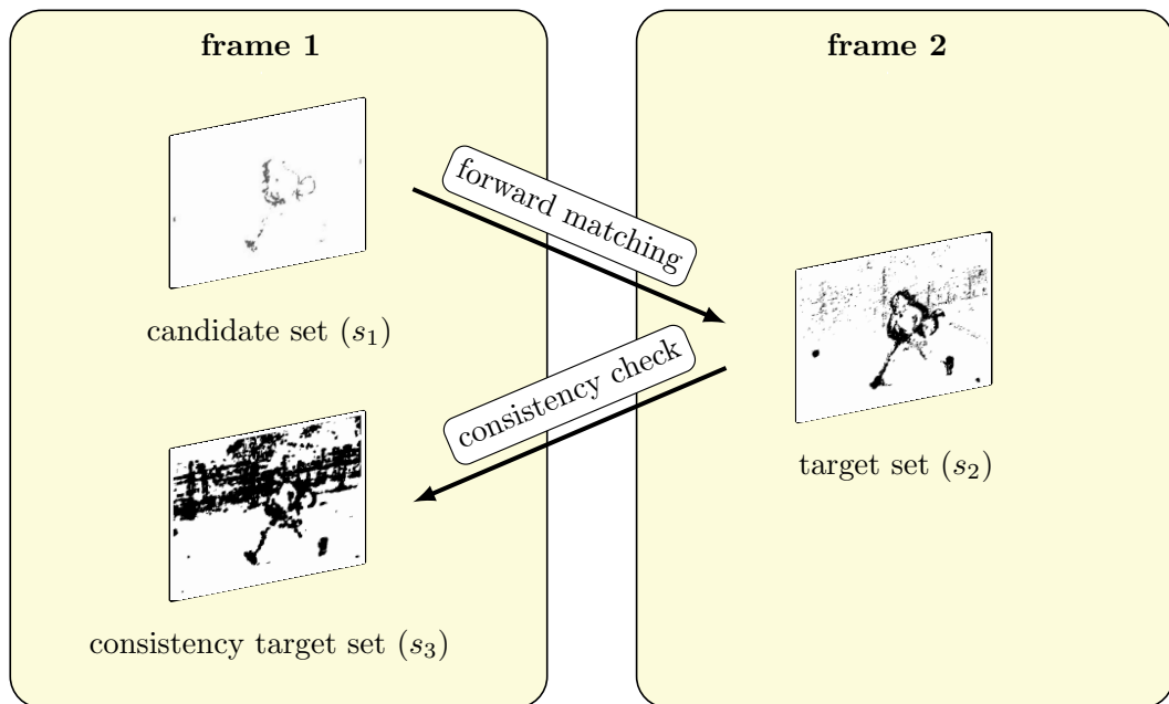
Figure 3.4: Illustration of the subsequent sets of locations during the matching process with a forward-backward consistency check (considered pixels are black). The sparsification reduces the runtime while the increasing size of the sets supports the consistency check to filter out unreliable matches.
