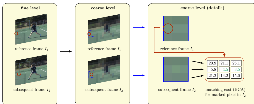
Figure 4.3: Illustration of the data costs at hand of the tennis ball of the Tennis sequence [27]. At the coarse level, the tennis ball is hardly distinguishable from the background but the displacement between the correct pixels still gives the least data costs.
