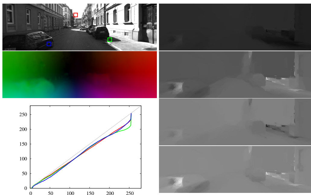
Figure 5.4: Estimated coefficients and BTFs. Left column, from top to bottom: Frame 1 of the KITTI 2012 training sequence #15 with three highlighted positions, the estimated optical flow field, a plot of the BTFs where the colors of the BTFs correspond to the colors of the corresponding highlighting boxes. Right column, from top to bottom: Estimated coefficient fields b_1 to b_4 . The depiction is centered w.r.t. a grey value of 127 which corresponds to a coefficient value of 0. Darker values denote negative coefficients, brighter values represent positive coefficients.
