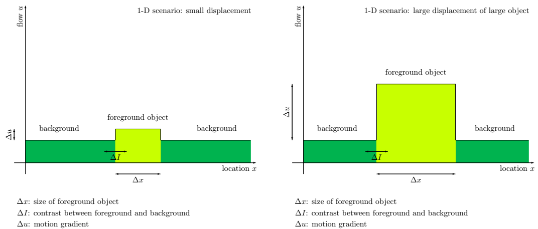
Figure 4.1: 1-D Illustrations of different displacement scales that can be handled by coarse-to-fine schemes. From left to right: Small displacement, large displacement of a large object.
