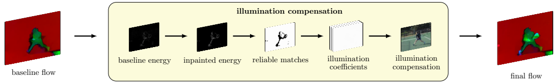
Figure 6.4: Detailed schematic overview of the partially decoupled method at hand of the Tennis sequence [27].
