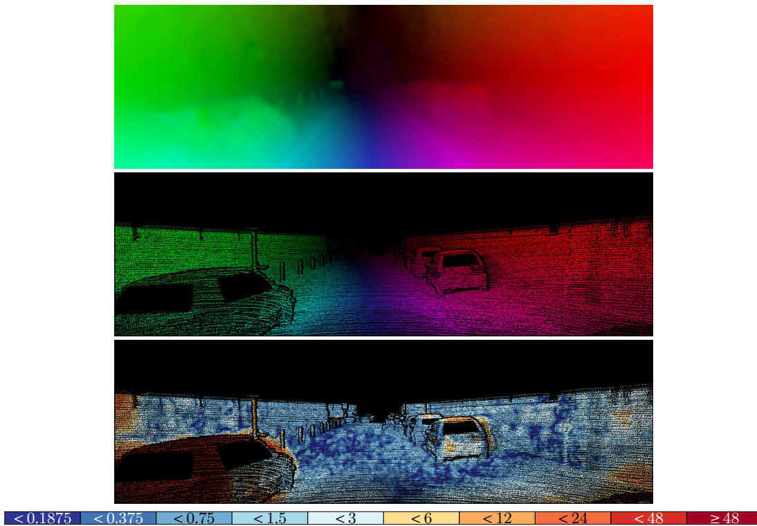
Figure 1.4: Exemplary illustration of the bad pixel visualization. Top: Estimated flow for Sequence 15 of the KITTI 2012 training data set. Center: Ground truth flow. Bottom: Bad pixel visualization for a threshold T = 3 . Blue regions indicate an endpoint error below the threshold T . In white regions it is close to but still smaller than T and in brown regions it is above T .
