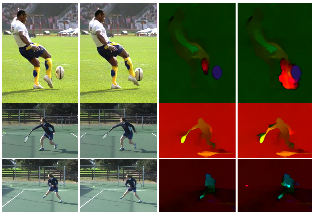
Figure 6.14: Results for further large displacement sequences. From Top to Bottom: Football [160], Tennis (Frame 502) [27], Tennis (Frame 577) [27]. From Left to Right: First frame, second frame, baseline, our method.
