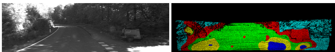
Figure 5.2: Exemplary depiction of the clusters of a coefficient field. Left: Frame 1 of the KITTI 2012 training sequence #114. Right: Resulting clusters of the K -Means algorithm. While black pixels indicate locations where no ground truth is provided, each color indicates a separate cluster. On the one hand, we can see the three red spots in the depiction that correspond to the inter-reflections at the windshield, while on the other hand, we observe different clusters for the street and the environment which are the result of a stronger brightening effect on the street in contrast to a weaker brightening in the environment.
