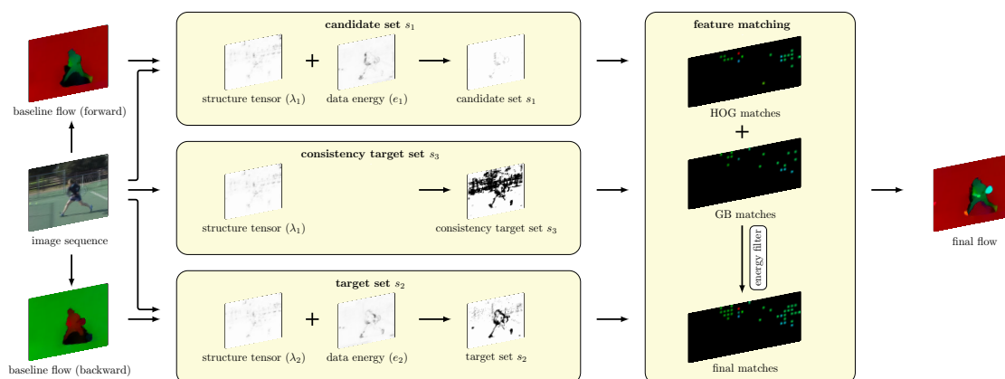
Figure 3.5: Detailed illustration of the flow estimation for Frame 496 of the Tennis sequence.
