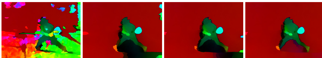
Figure 3.8: Results for the Tennis sequence (Frame 496) for different combinations of selection criteria and confidence strategies. From Left to Right: (a) No selection + uniform (46336 matches). (b) Structure + uniqueness (9573 matches). (c) Energy + energy (1220 matches). (d) Both + both (only 734 matches).
