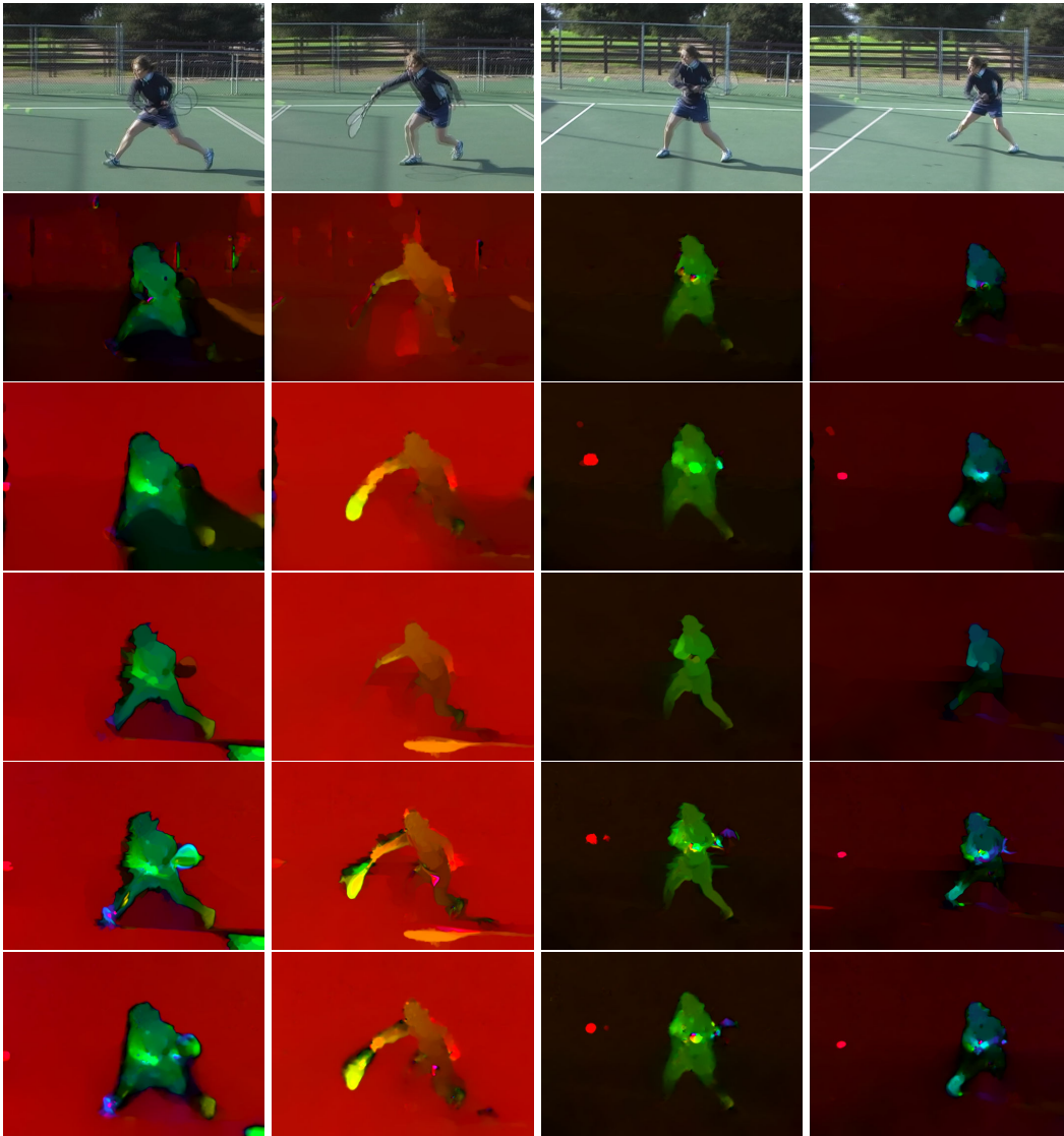
Figure 4.8: Comparison of LDOF and our method with the corresponding baseline results. Left to right: Tennis sequences 496, 502, 538, 577 [27]. Top to down: Overlaid frames, LDOF baseline, LDOF, our baseline, our result, our result (LDOF regularizer).
