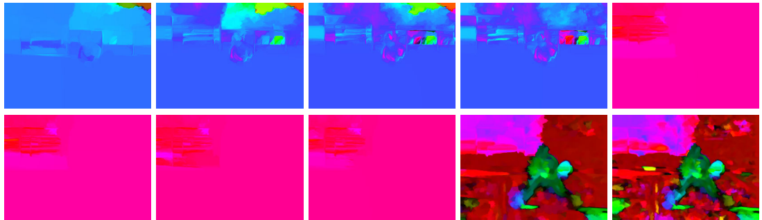
Figure 6.12: Flow candidates for the Tennis sequence with artificial illumination changes when illumination compensation is deactivated. First row: BCA data term, candidate sets one to five. Second row: BCA data term, candidate sets six to eight, and GBCA data term, candidate sets one and two.
