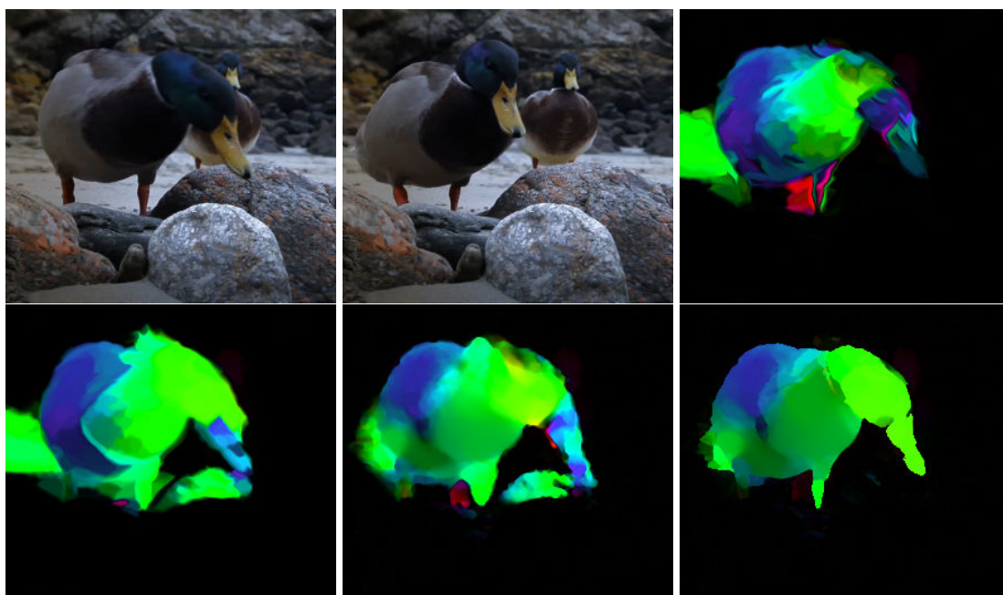
Figure 6.17: Limitations of our method at hand of the Bird sequence [160]. From left to right, top to bottom: First frame, second frame, baseline, our method, MDP-Flow without occlusion handling, MDP-Flow with occlusion handling [160].
