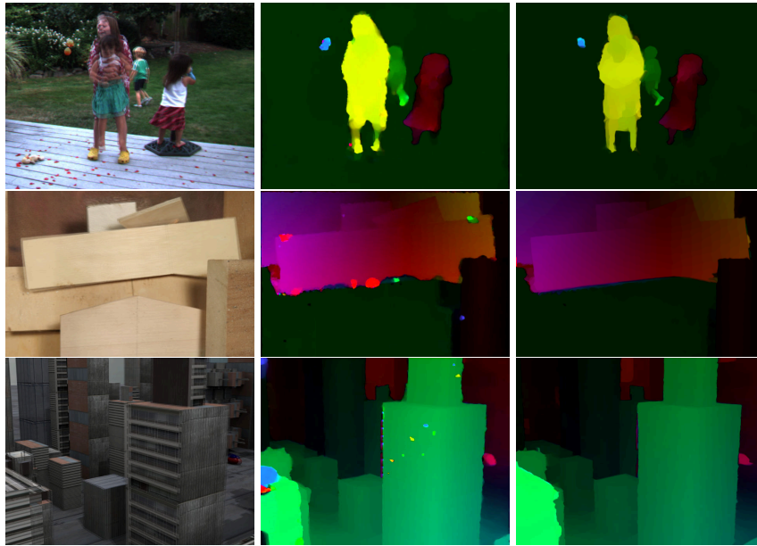
Figure 3.7: Comparison between LDOF and ALD-Flow with respect to outliers for some sequences from the Middlebury benchmark. From top to down: Backyard, Wooden and Urban. From left to right: Overlaid frames, LDOF, ALD-Flow .
