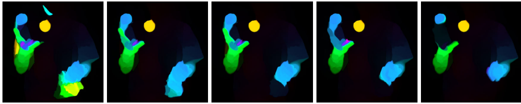
Figure 3.9: Evaluation of the sensitivity of the threshold parameters for the Beanbags sequence (zoom-ins). From Left to Right: All thresholds changed to (a) 40 percent, (b) 80 percent, (c) 100 percent, (d) 120 percent, (e) 160 percent of the optimal value.
