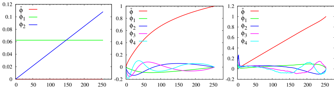
Figure 5.1: Comparison of different basis functions. From left to right: (a) Normalized affine basis. (b) EMoR functions [57]. (c) Our basis functions learned from KITTI ground truth data.
