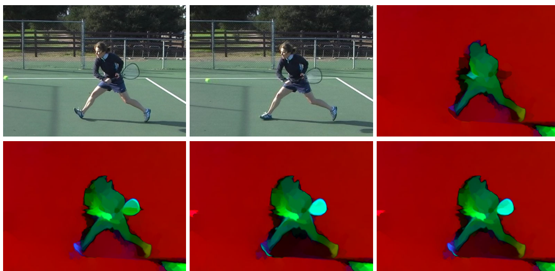
Figure 6.10: Influence of the candidate flows. First row, from left to right: First frame, second frame, baseline result. Second row, from left to right: Our result using proposals from only the BCA data term, only the GBCA data term, both data terms.
