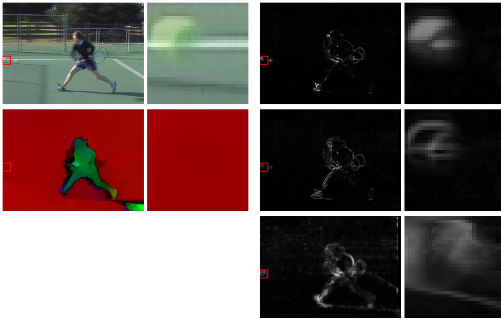
Figure 6.2: Comparison of data term energies (with zoom-ins) for different constancy assumptions evaluated on the same baseline flow for the Tennis sequence. Left column: Overlaid input frames, baseline flow field. Right column: Data energies evaluated using the BCA, GCA and Geometric Blur constancy. Higher intensity denotes a higher data energy.
