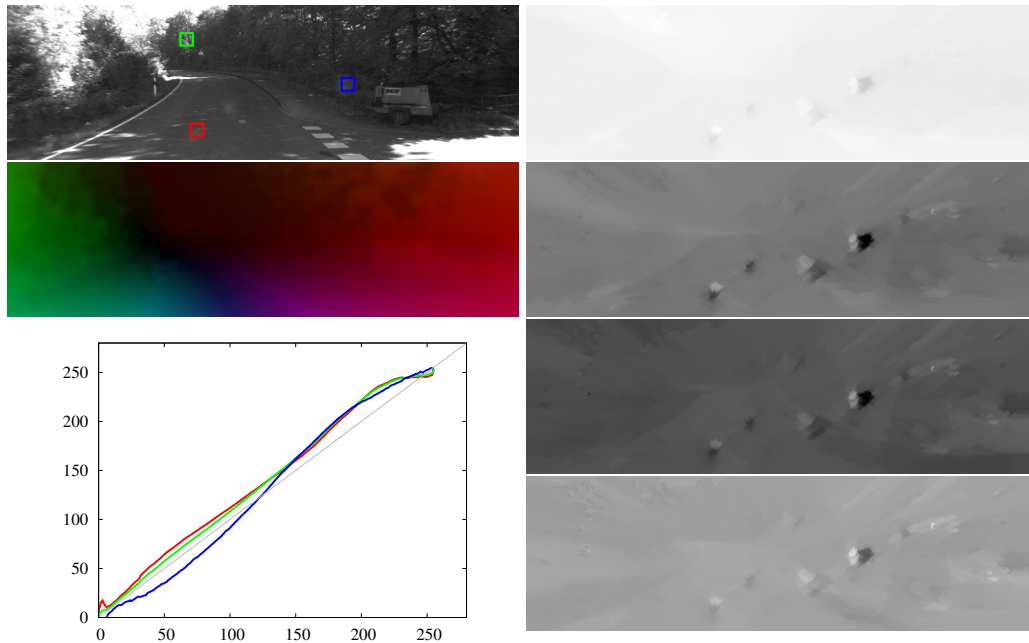
Figure 5.5: Estimated coefficients and BTFs. Left column, from top to bottom: Frame 1 of the KITTI 2012 training sequence #114 with three highlighted positions, the estimated optical flow field, a plot of the BTFs where the colors of the BTFs correspond to the colors of the corresponding highlighting boxes. Right column, from top to bottom: Estimated coefficient fields b_1 to b_4 . The depiction is centered w.r.t. a grey value of 127 which corresponds to a coefficient value of 0. Darker values denote negative coefficients, brighter values represent positive coefficients.
