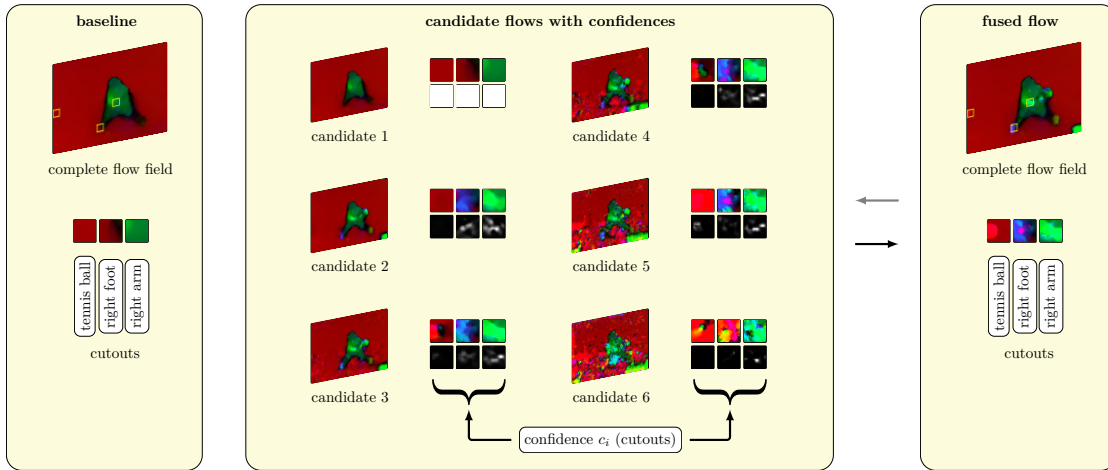
Figure 4.4: Illustration of the results for a decreasing smoothness weight with confidence functions and the fused result. Brighter areas in the confidence visualizations denote higher values.
